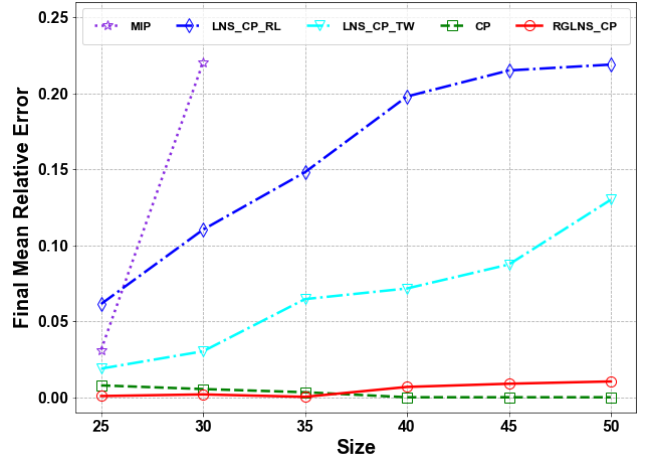
Figure 4: Final MRE of square JSP instances.
