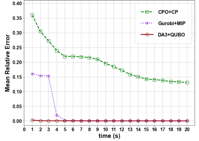
Figure 6: MRE of one-machine scheduling problems.
