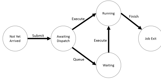
Fig. 3: Stages of job lifetime.
